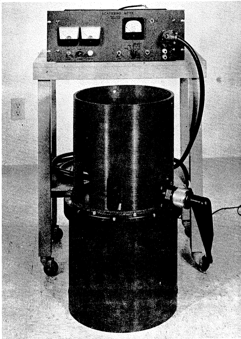
Figure 4. General Angle Scattering Meter.
